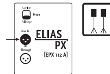
Anschluss-Schema Fullrange-Setup
